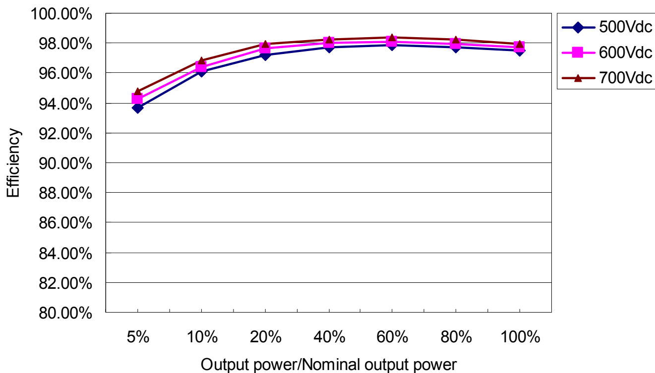
Efficiency curve
