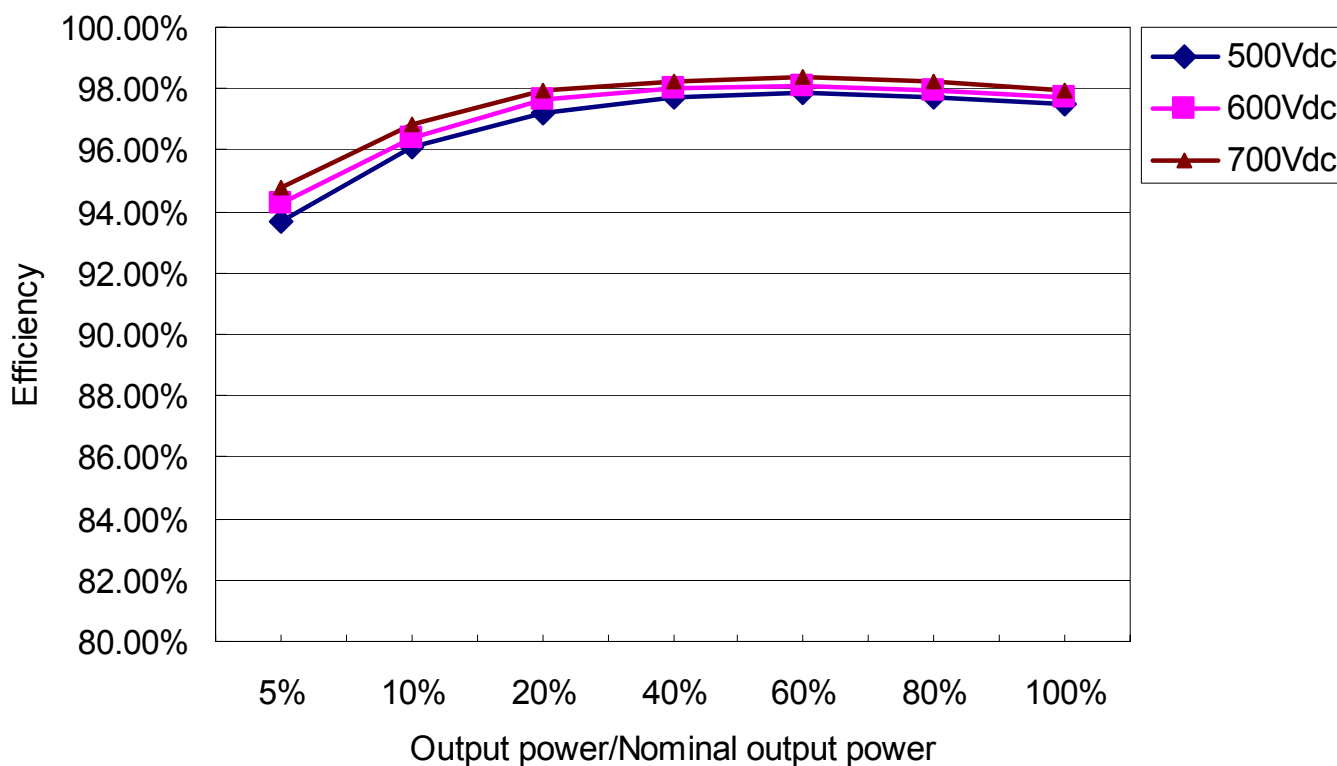
Efficiency curve
