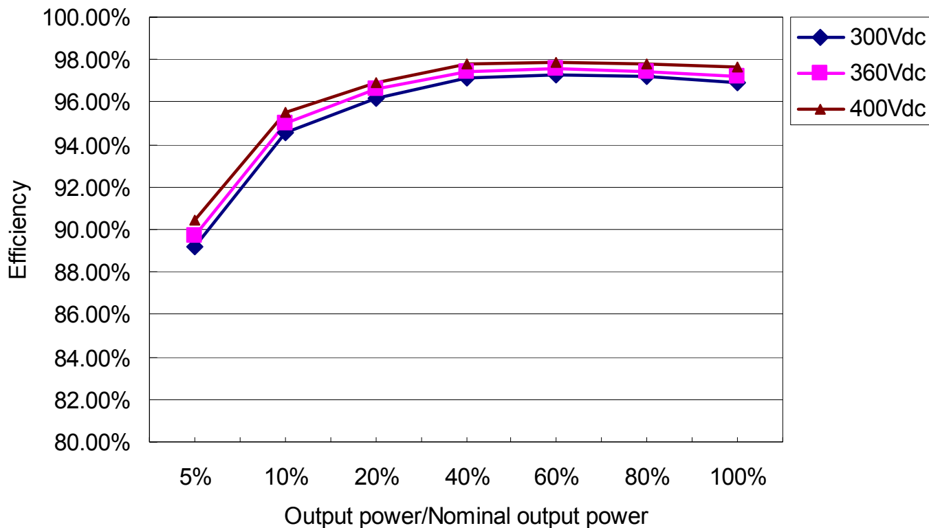
Efficiency curve
